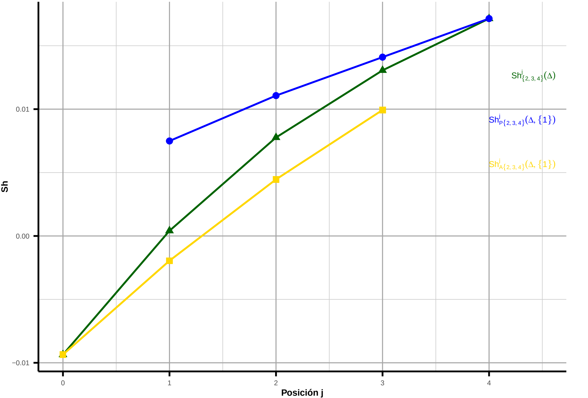
Influencia de Age [1] sobre Cho + Rac + Ris [2,3,4] (instancia fila = 1)
