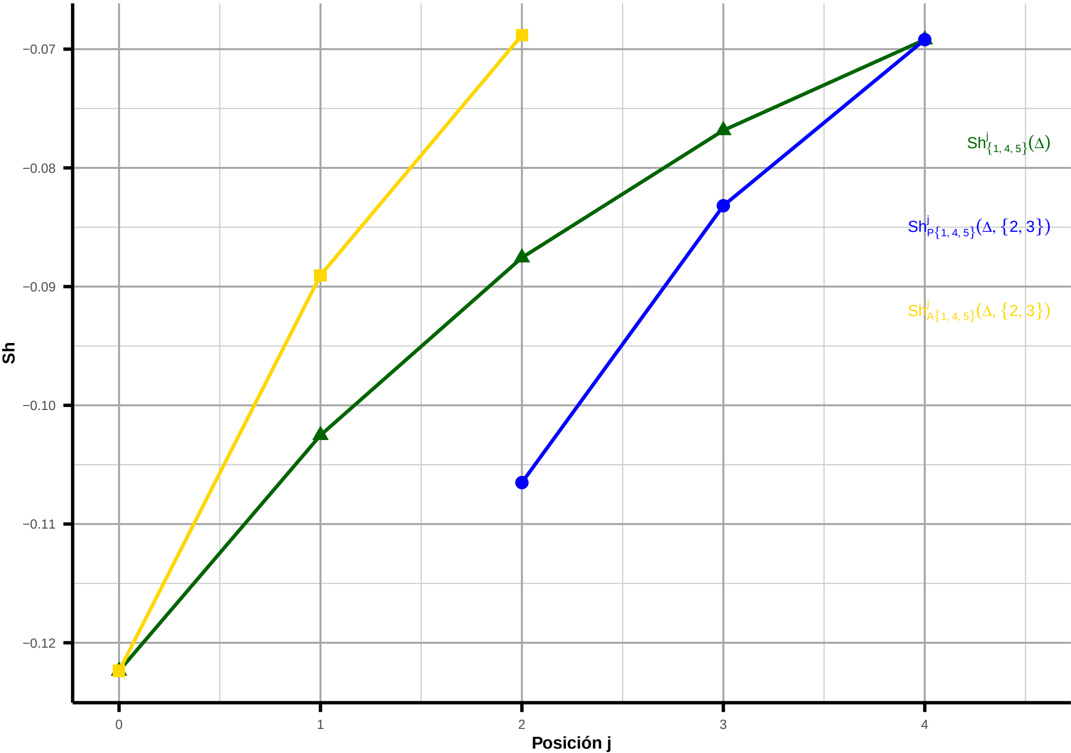
Influencia de Cho + Rac [2,3] sobre Age + Ris + Sex [1,4,5] (instancia fila = 1)
